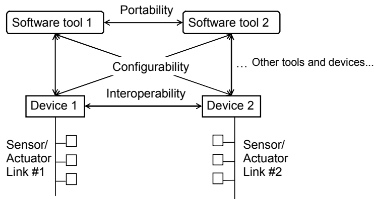
Figure 1 – Topics addressed by compliance profiles
