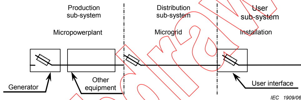
Figure 1 – General configuration of an electrification system
