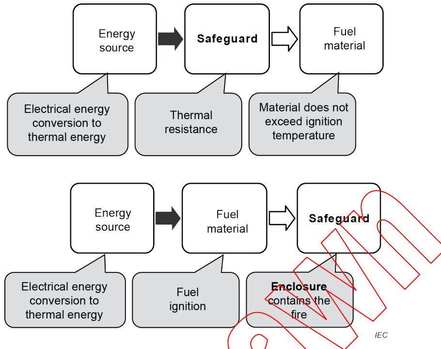
Figure 6 – Models for protection against fire
