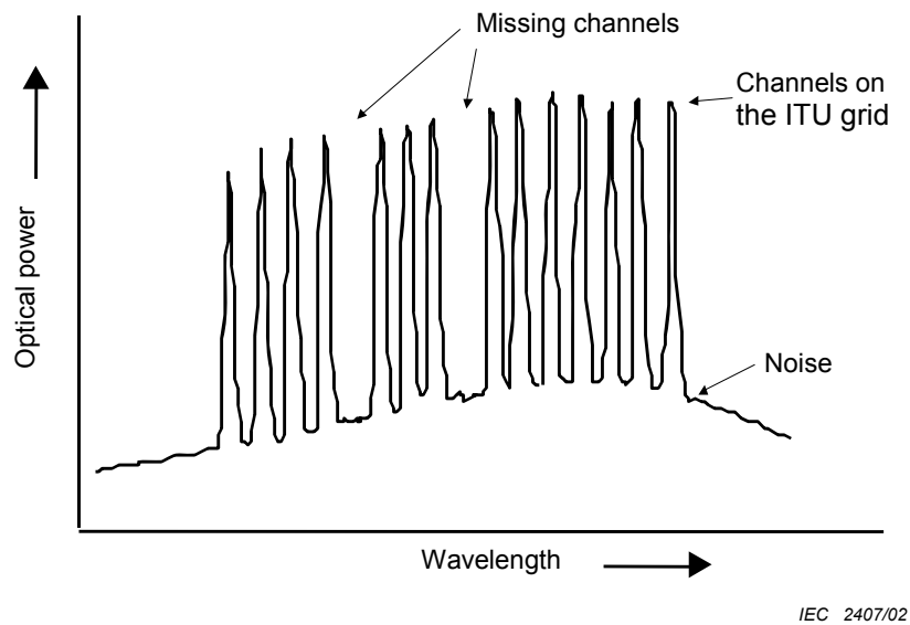
Figure 1 – Typical optical spectrum at an optical interface in a multichannel transmission system
