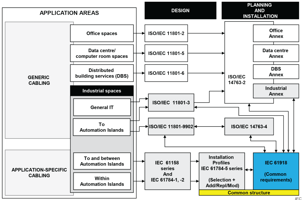
Figure 1 – Standards relationships
